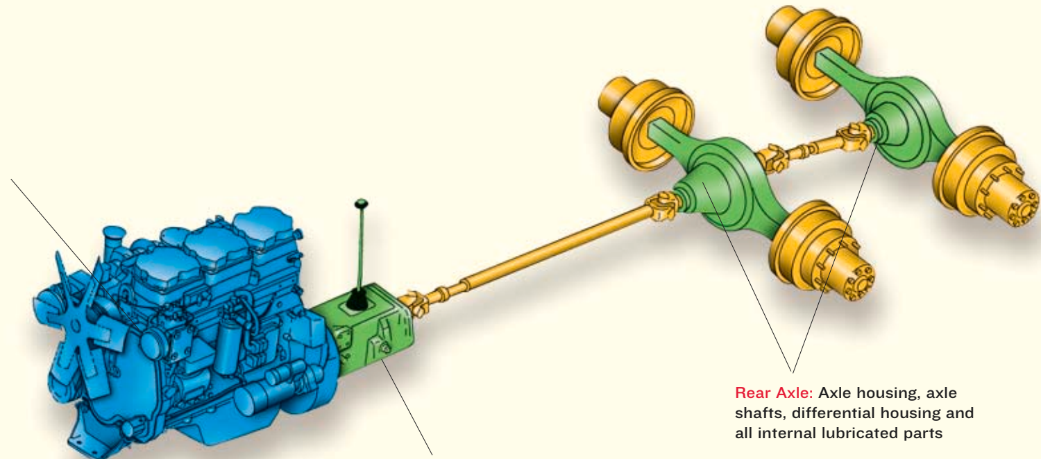
Transmission: Transmission housing and all internal lubricated parts
